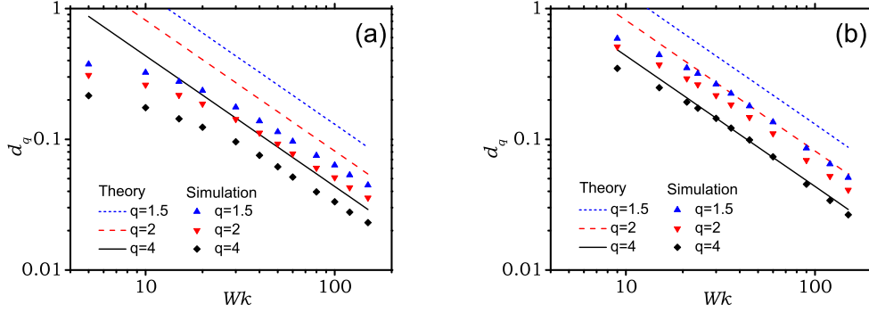
Figure 4.8: The anomalous dimensions d_q extracted from direct numerical diagonalization (symbols) for three different values of q are compared with the perturbation results (lines) of Eq. (4.17) in the weak coupling regime for different values of disorder and (a) k = 1 or (b) k = 3 . The numerical results converge to the theory slowly.
