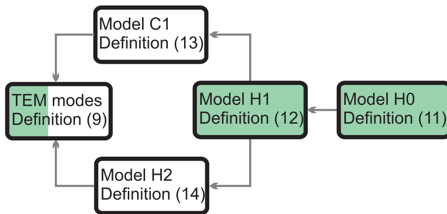
Figure 4.10: Summary of the scaling analysis on PDF of eigenvectors of matrices from various models. The intermediate hypothetic models transform the Hermitian RBM to the model describing TEM coupling. The colored boxes indicate those models that show critical scaling behavior. The model indicated by white boxes have localized eigenvectors. For TEM modes, only a part of the spectrum is critical.
