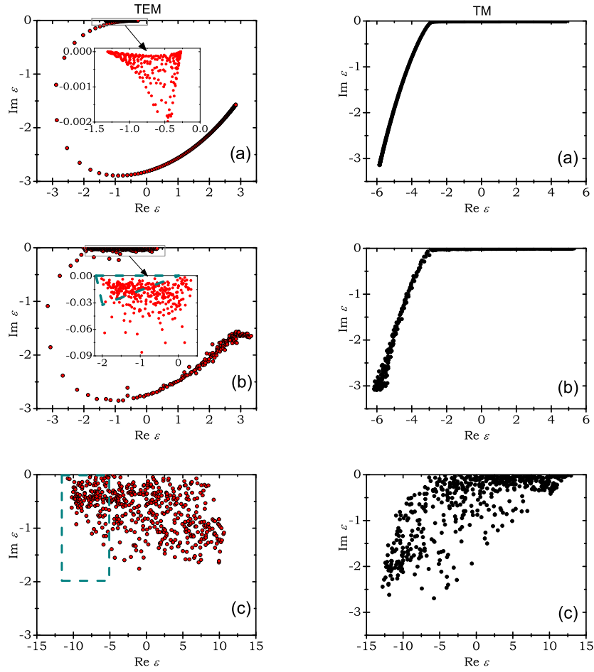
Figure 4.1: Left column: complex valued spectrum of the TEM interaction matrix (4.9) with k = 1 for (a) homogeneous ( W = 0 ) and disordered in regimes of (b) strong ( W = 2 ) and (c) weak ( W = 20 ) coupling. The dashed square in (c) shows the region where the corresponding TEM eigenmodes are scaling critically. The eigenmodes corresponding to the eigenvalues in the dashed regions are selected for further statistical analysis. Right column: same as the left for TM polarization.
