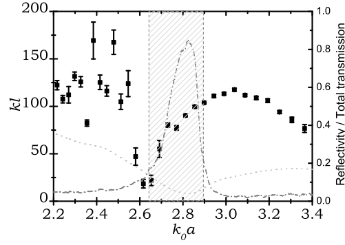
Figure 6.2: Optical characterization of opal photonic crystals. The dots show the scattering parameter k\ell as a function of frequency. The dashed line is the specular reflection at normal incidence and the dotted line is the total transmission of light impinging at normal incidence, which is measured by using an integrating sphere. The gray shaded area indicates the stop band.
